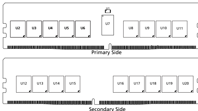
Figure 1: 288-Pin RDIMM (R/C-C3)
