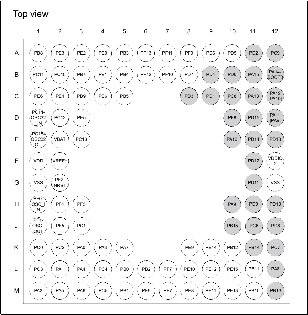
Figure 4. STM32G0C1Vxl UFBGA100 pinout
