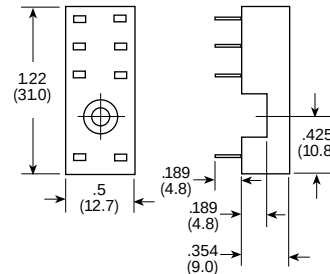
Hold-Down Spring RP16041
