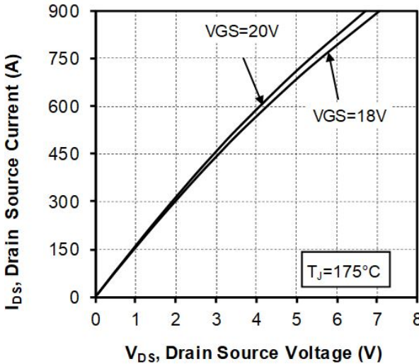
Figure 1-3. Output Characteristics, T J = 175 °C
