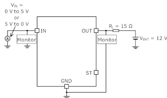
Measurement Circuit for Figure 10, Figure 11, Figure 12, Figure 13, Figure 14, Figure 15, Figure 16, Figure 17
