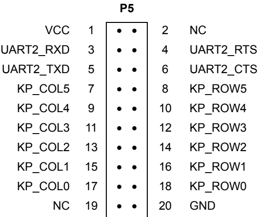
Figure 3-13. External Keypad Connector P5 Pin Assignments
