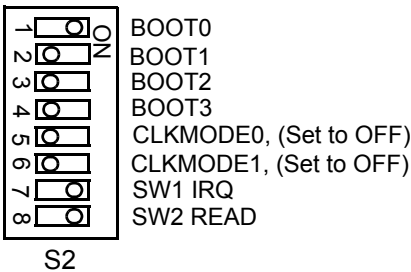
Figure 2-2. Switch S2
