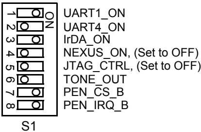
Figure 2-1. Switch S1
