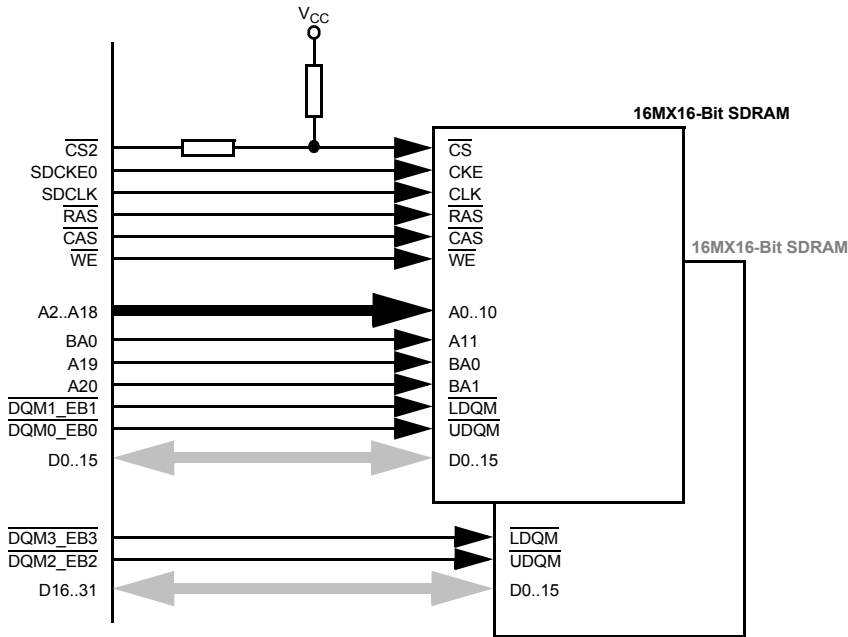
Figure 2-5. SDRAM Interface
