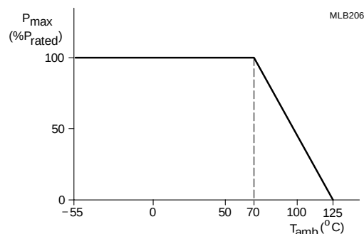
Fig. 13 Maximum dissipation (P) in percentage of rated power as a function of the operating ambient temperature (T amb )
