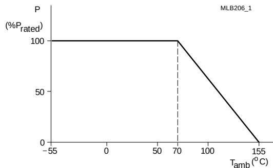
Fig. 14 Maximum dissipation (P) in percentage of rated power as a function of the operating ambient temperature (T amb )
