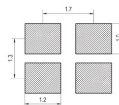
Figure 2) Suggested land pattern
