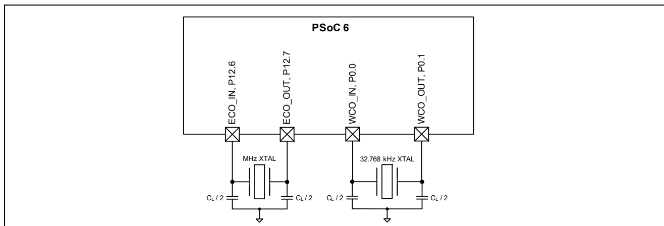
Figure 5 Oscillator circuits
