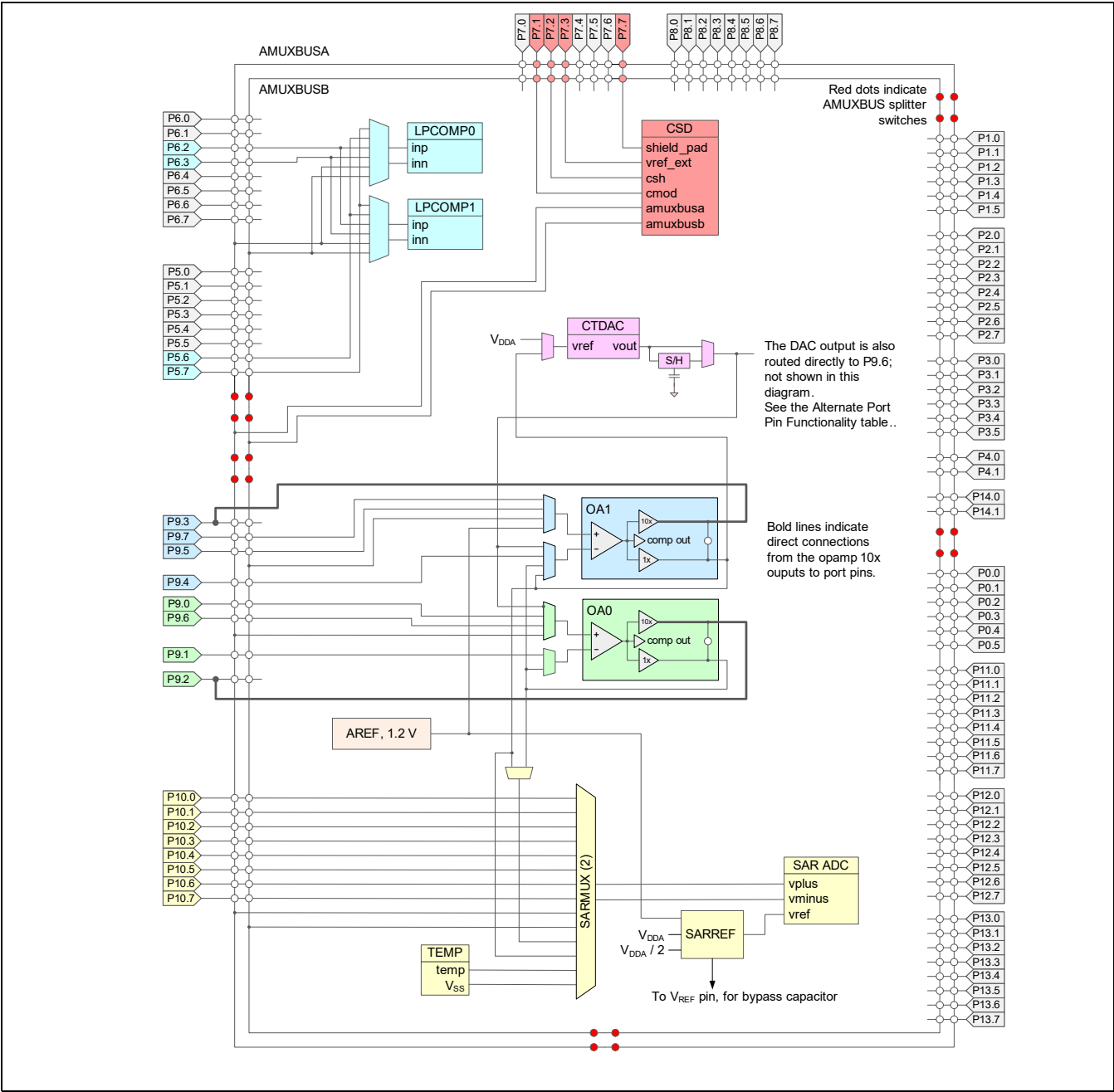
Figure 7 Analog subsystem
