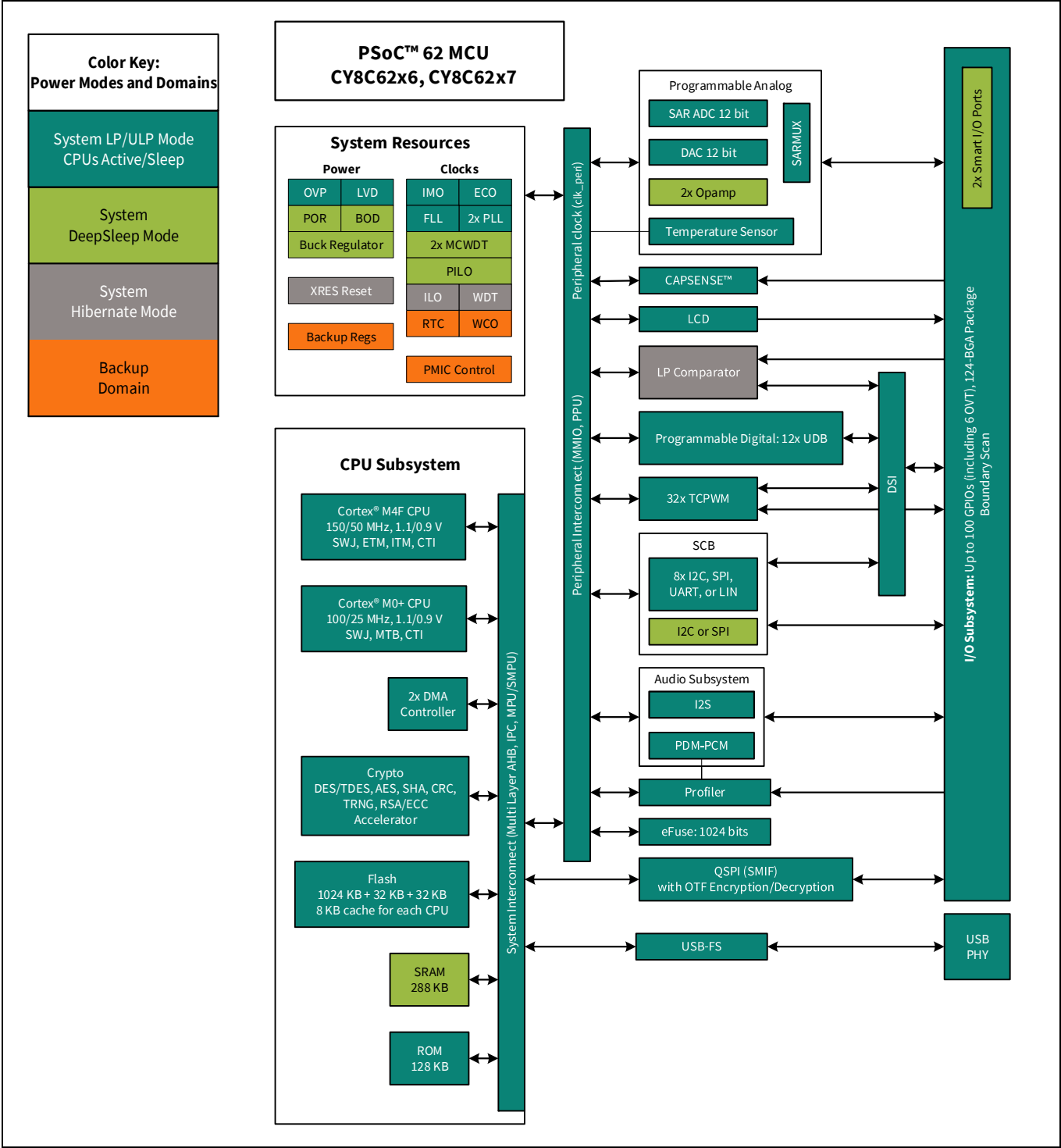
Figure 3 Block diagram
