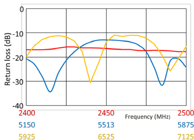
Return Loss
