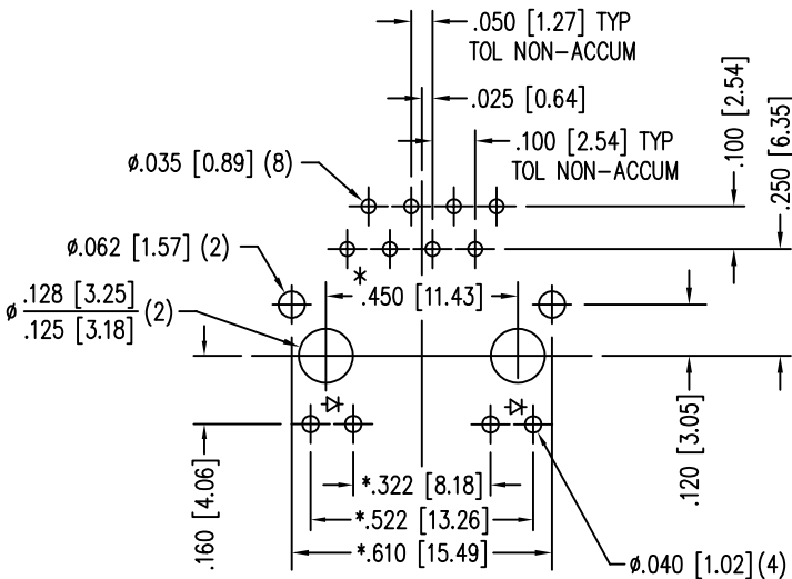
P.C.B. RECOMMENDED HOLE LAYOUT SEEN FROM COMPONENT SIDE TOLERANCE \pm 0.003 [0.08] UNLESS OTHERWISE SPECIFIED
