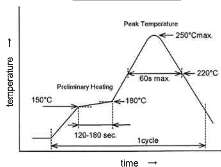
Reflow temperature profile
