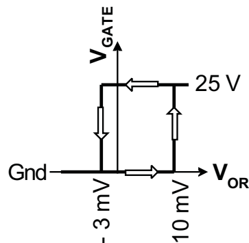
Figure 24. ORing Thresholds
