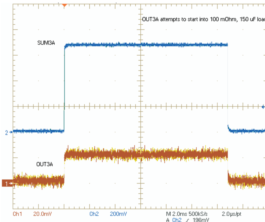
Figure 14. OUT3A Startup Into Short Circuit
