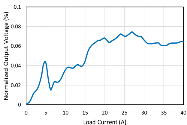
EM2140 Load Regulation, V_{OUT} = 0.9V
