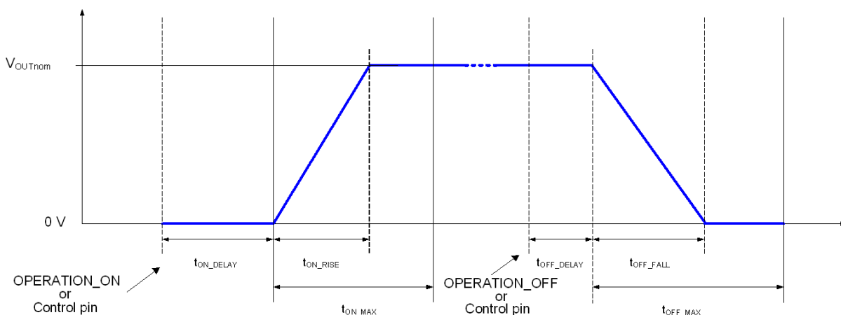
Figure 6: Power Sequencing
