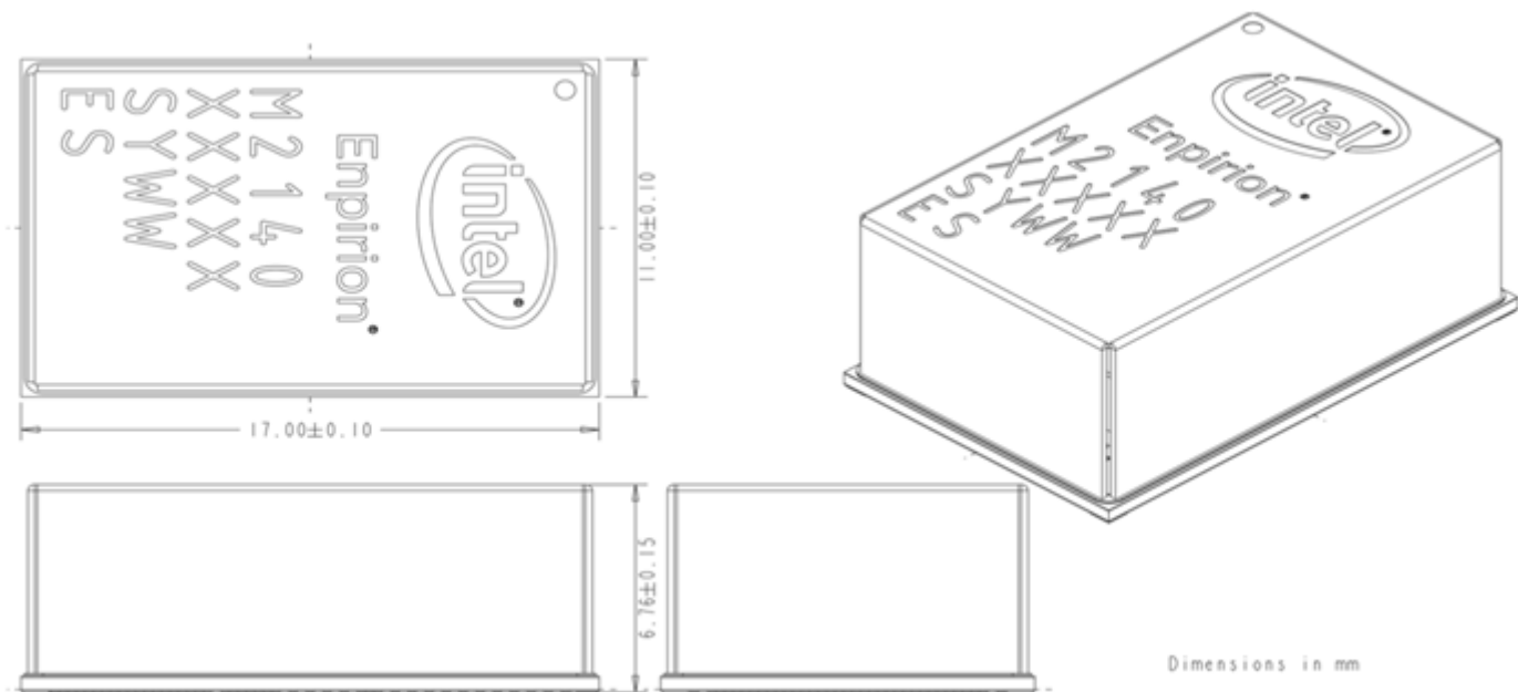
Figure 23: Package Dimensions
