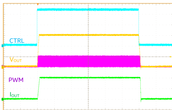
Start-up/Shutdown, CTRL At 20A Load, 10 ms/div
