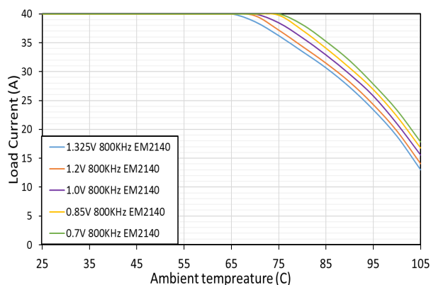
Thermal Derating, No Airflow
