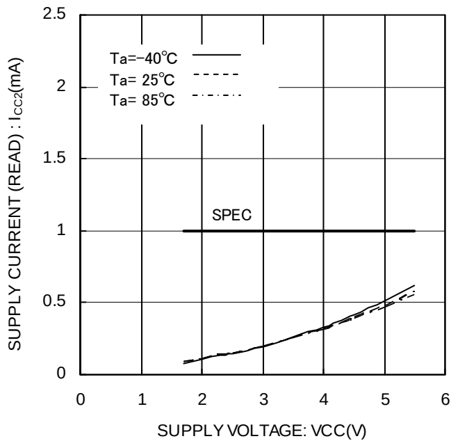
Figure 16. Supply current (READ) I_{CC2}(\text{READ}, f_{SK}=3\text{MHz})
