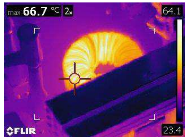
Figure 21: Thermal scan of Inductor (650V)
