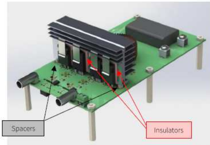
Figure 7: Mechanical assembly
