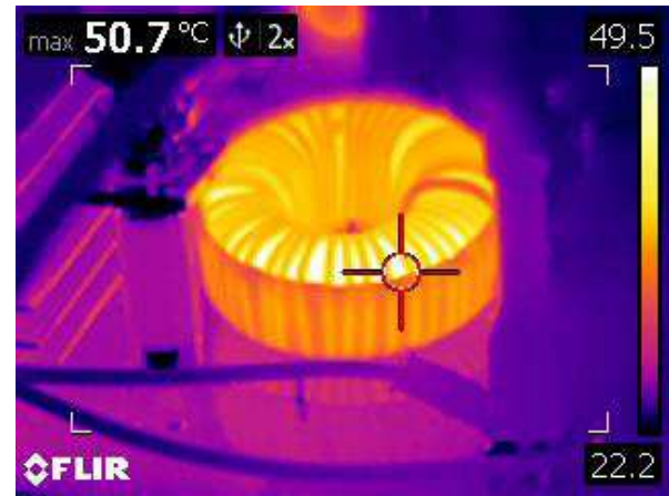
Figure 19: Thermal scan of Inductor (1200V)
