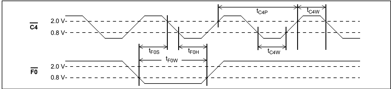
Figure 16 - C4 Clock & Frame Pulse Alignment for ST-BUS Streams in DN Mode
