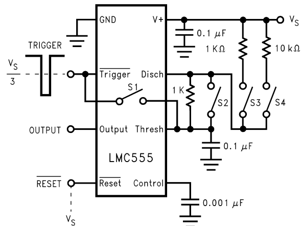
Figure 6-1. Test Circuit
