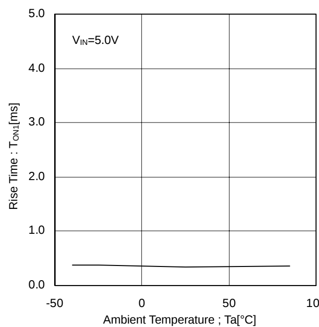
Figure 21. Output Rise Time
