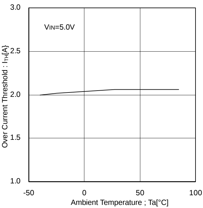
Figure 15. Over-Current Threshold
