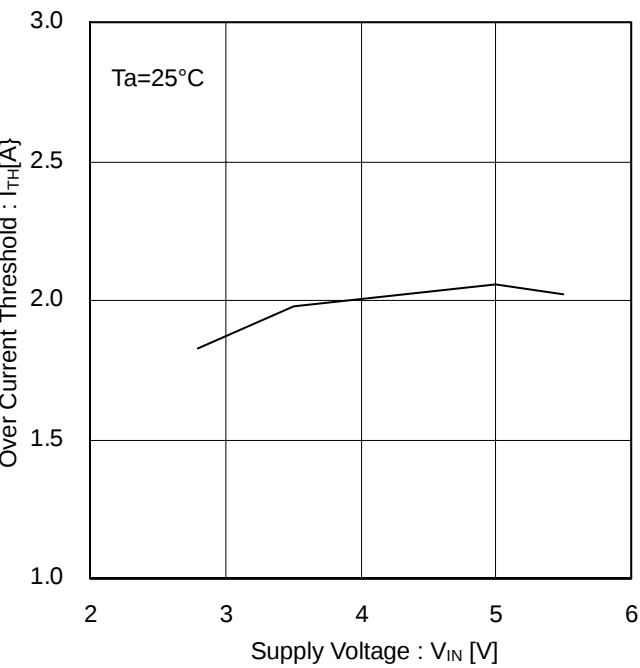
Figure 14. Over-Current Threshold
