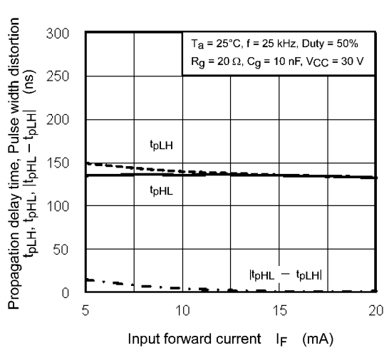
Fig. 12.2.13 t_{pLH}, t_{pHL}, |t_{pHL} - t_{pLH}| - I_F
