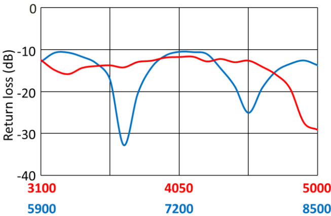
Return Loss
