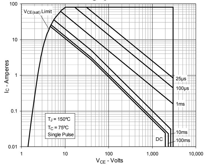
Fig. 20. Forward-Bias Safe Operating Area
