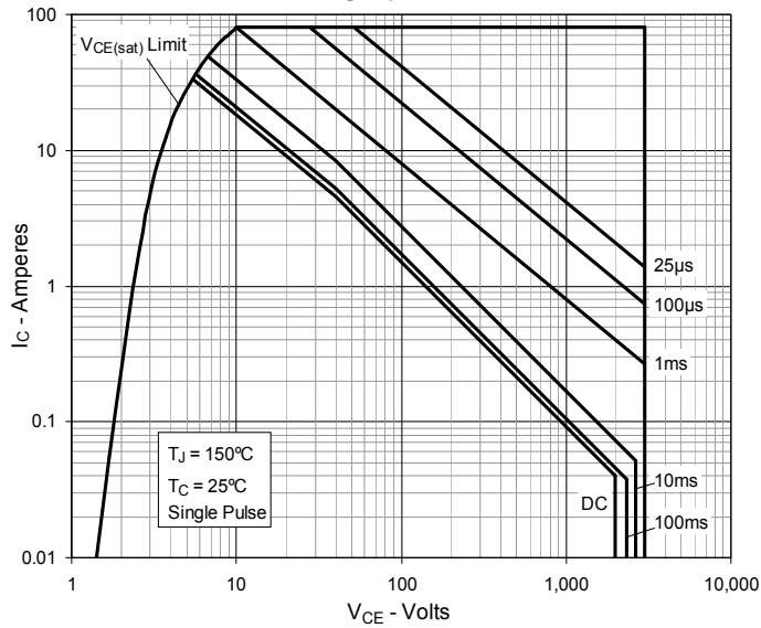
Fig. 19. Forward-Bias Safe Operating Area
