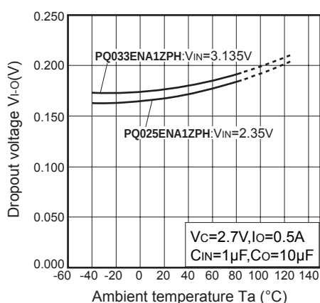
Fig.11 Dropout Voltage vs. Ambient Temperature (PQ025ENA1ZPH, PQ033ENA1ZPH)
