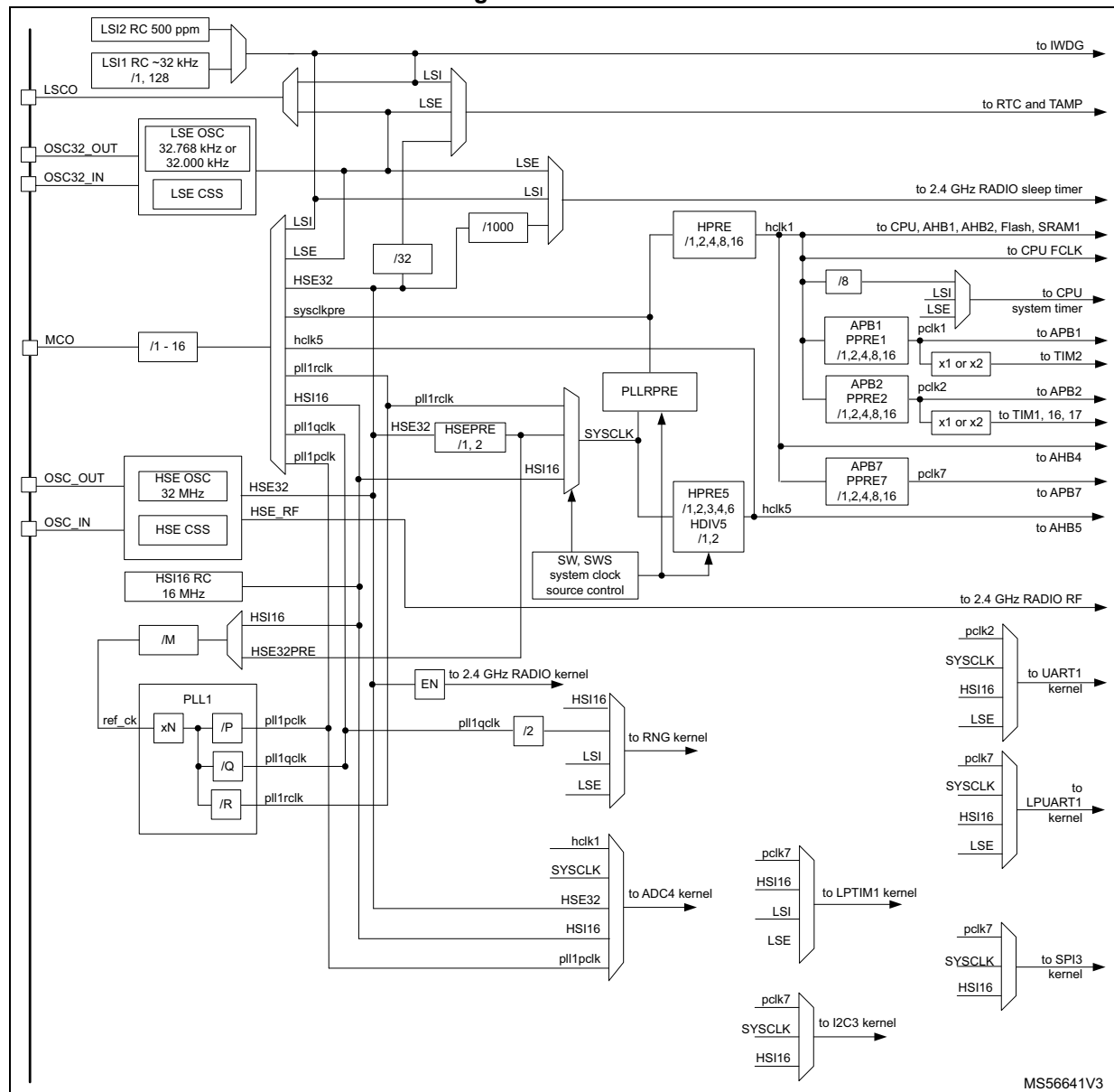
Figure 5. Clock tree
