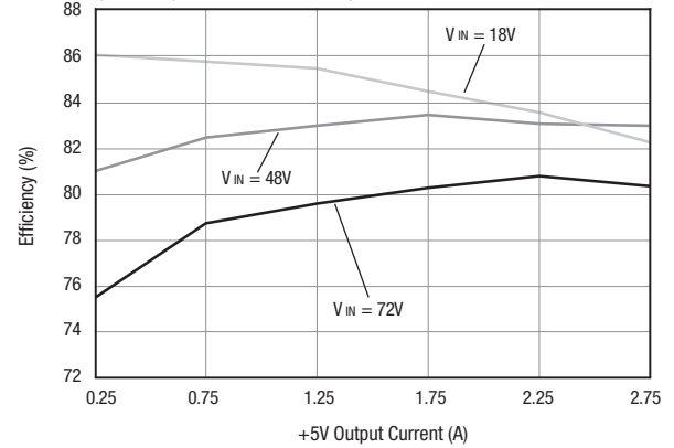
Efficiency vs. +5V Output Loading
