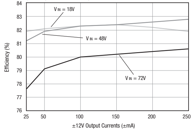
Efficiency vs. \pm 12\text{V} Output Loading
