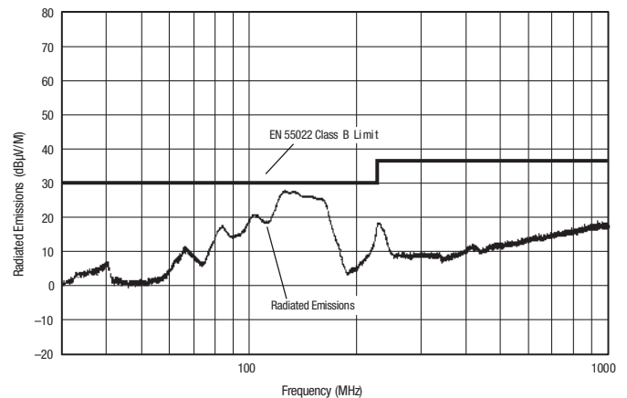
TWR-5/3000-15/500-D12A Radiated Emissions EN 55022 Class B, 10 Meters Converter Output = +5Vdc @ 2.7A and \pm 15Vdc @ \pm 450mA
