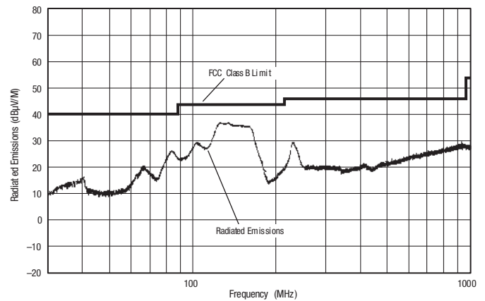
TWR-5/3000-15/500-D12A Radiated Emissions FCC Part 15 Class B, 3 Meters Converter Output = +5Vdc @ 2.7A and \pm 15Vdc @ \pm 450mA
