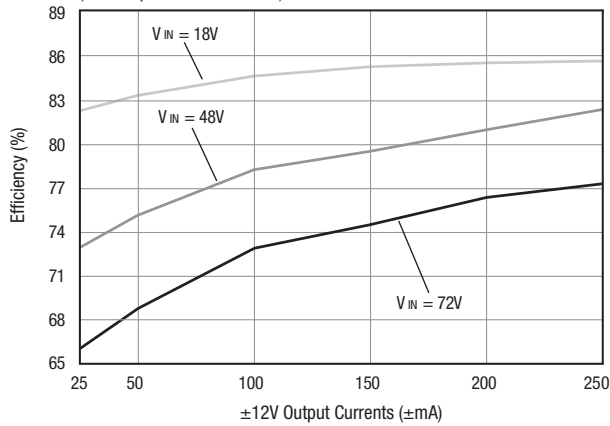
Efficiency vs. \pm 12\text{V} Output Loading
