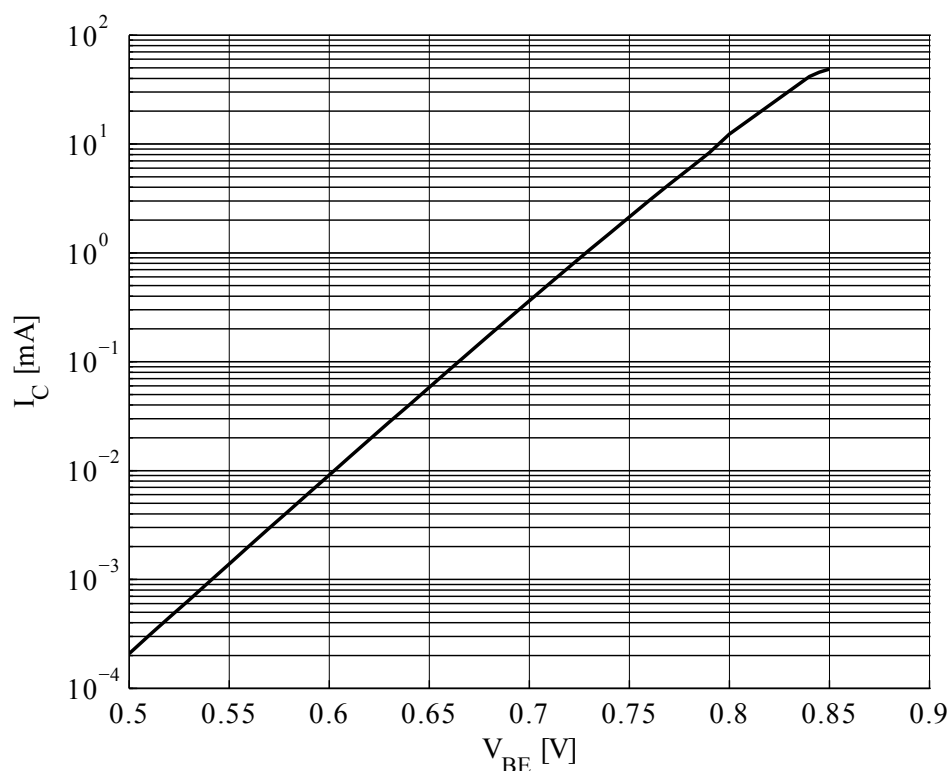
Figure 5 Collector current vs. base emitter forward voltage I_C = f(V_{BE}) , V_{CE} = 2\text{ V}
