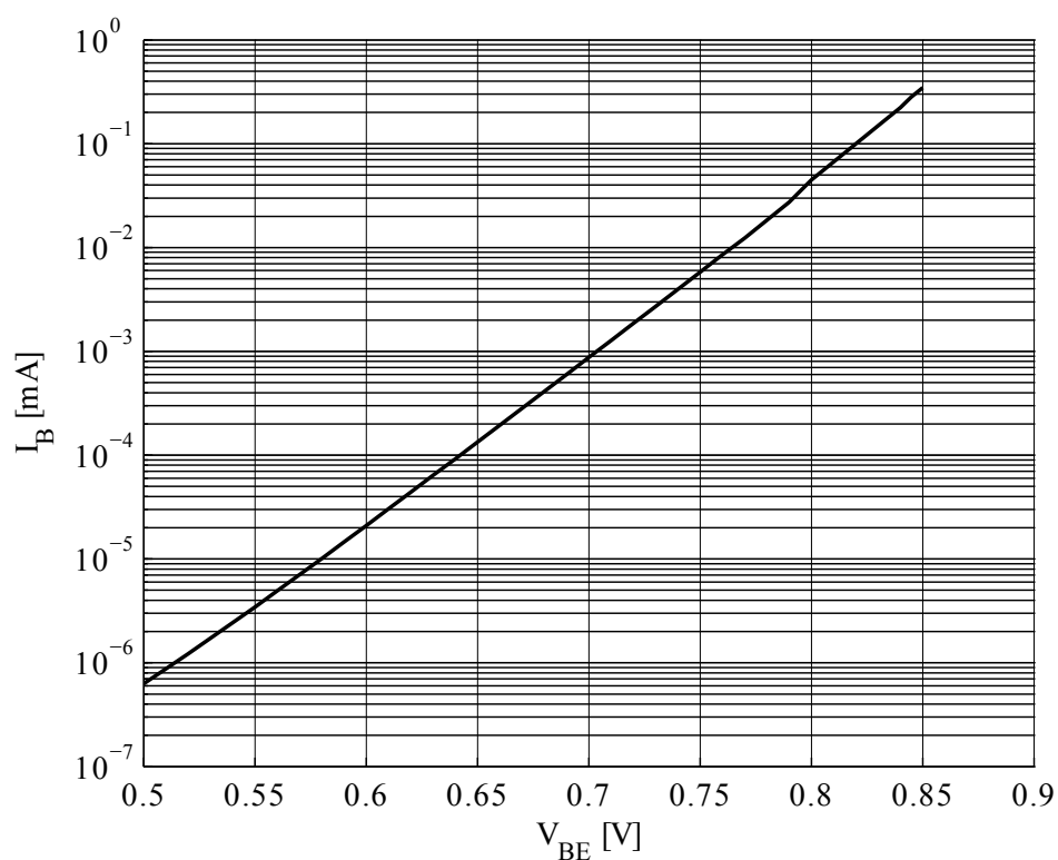
Figure 6 Base current vs. base emitter forward voltage I_B = f(V_{BE}) , V_{CE} = 2\text{ V}
