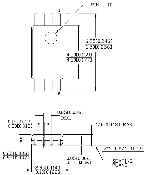
Figure 7. 8-pin TSSOP (4.40 mm Body) Z08.173/ZZ08.173 Package Outline, 51-85093
