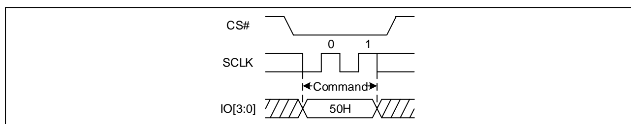
Figure 18 Write Enable for Volatile Status Register Sequence Diagram (QPI)
