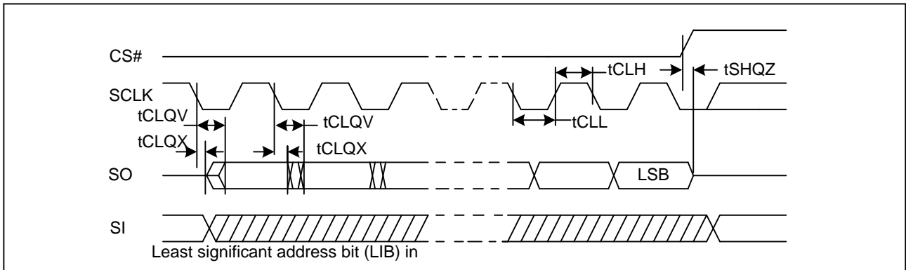
Figure 94. Output Timing
