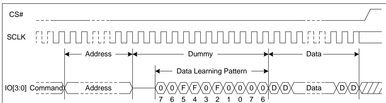
Figure 5. Data Learning Pattern Sequence Diagram (STR, Dummy Clock \geq 10 )
