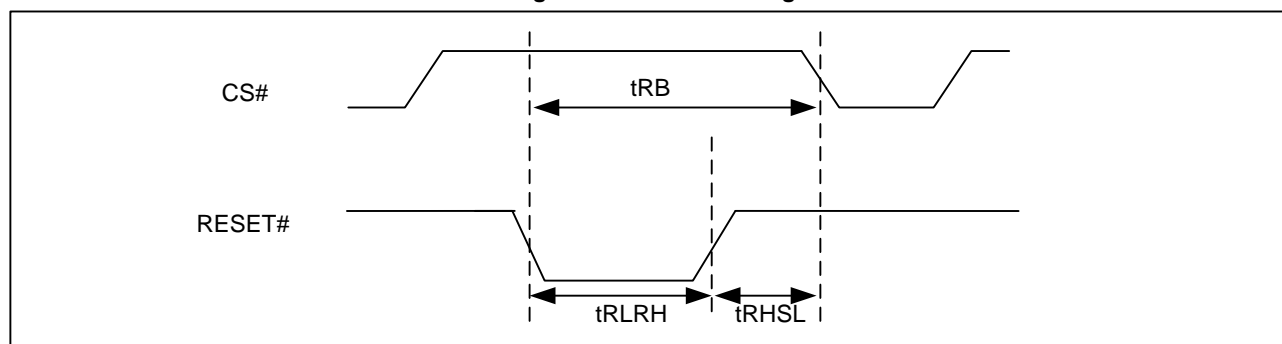
Figure 99. RESET Timing
