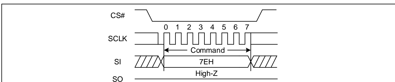
Figure 82 Global Block/Sector Lock Sequence Diagram (SPI)
