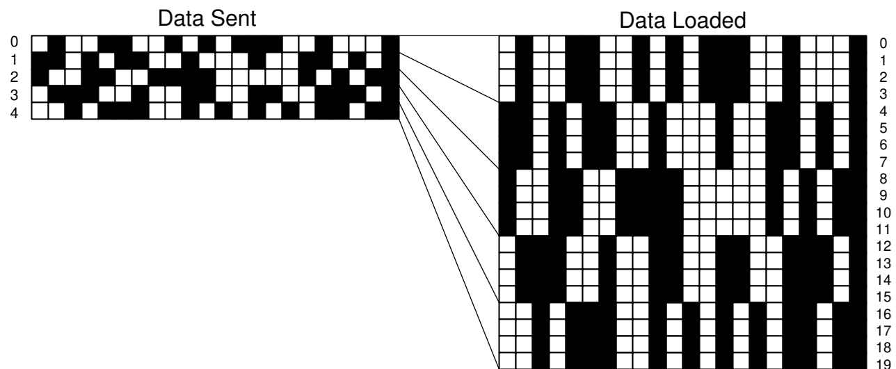
Figure 7-3. Example Load4 Row Address Mapping
