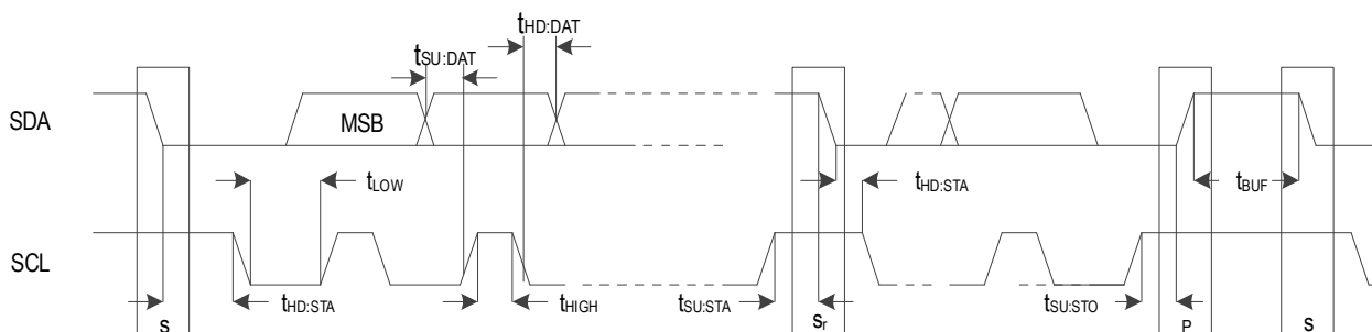
Figure 11. SMBus Target Timing Diagram
