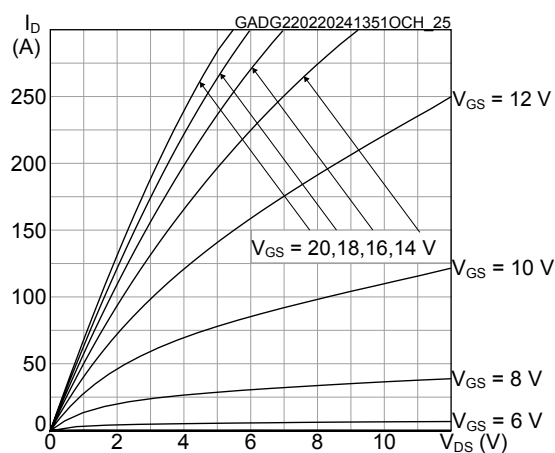
Figure 3. Typical output characteristics ( T_J = 25\text{ °C} )
