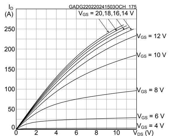
Figure 4. Typical output characteristics ( T_J = 175\text{ °C} )
