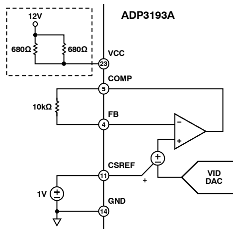
Figure 6. Positioning Voltage
