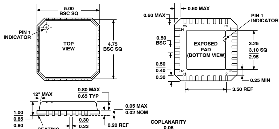
COMPLIANT TO JEDEC STANDARDS MO-220-VHDD-2 Figure 18. 32-Lead Lead Frame Chip Scale Package [LFCSP_VQ] 5 mm x 5 mm Body, Very Thin Quad (CP-32-2) Dimensions shown in millimeters
