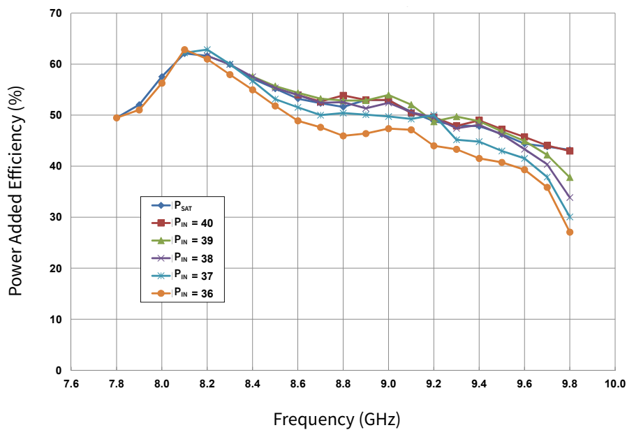
Figure 8. Power Added Efficiency vs Input Power & Frequency V_{DD} = 40 V, P_{IN} = 39 dBm, Duty Cycle = 10%
