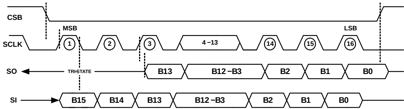
Figure 13. SPI Timing diagram
