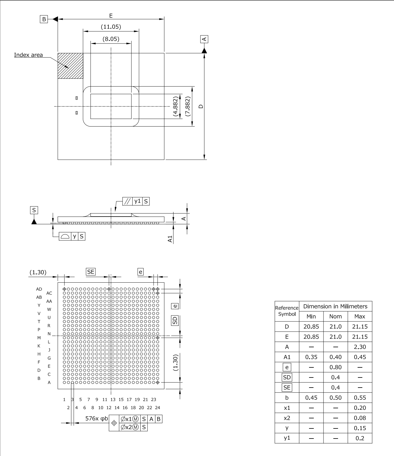
Figure A1.2 576-pin FCBGA
