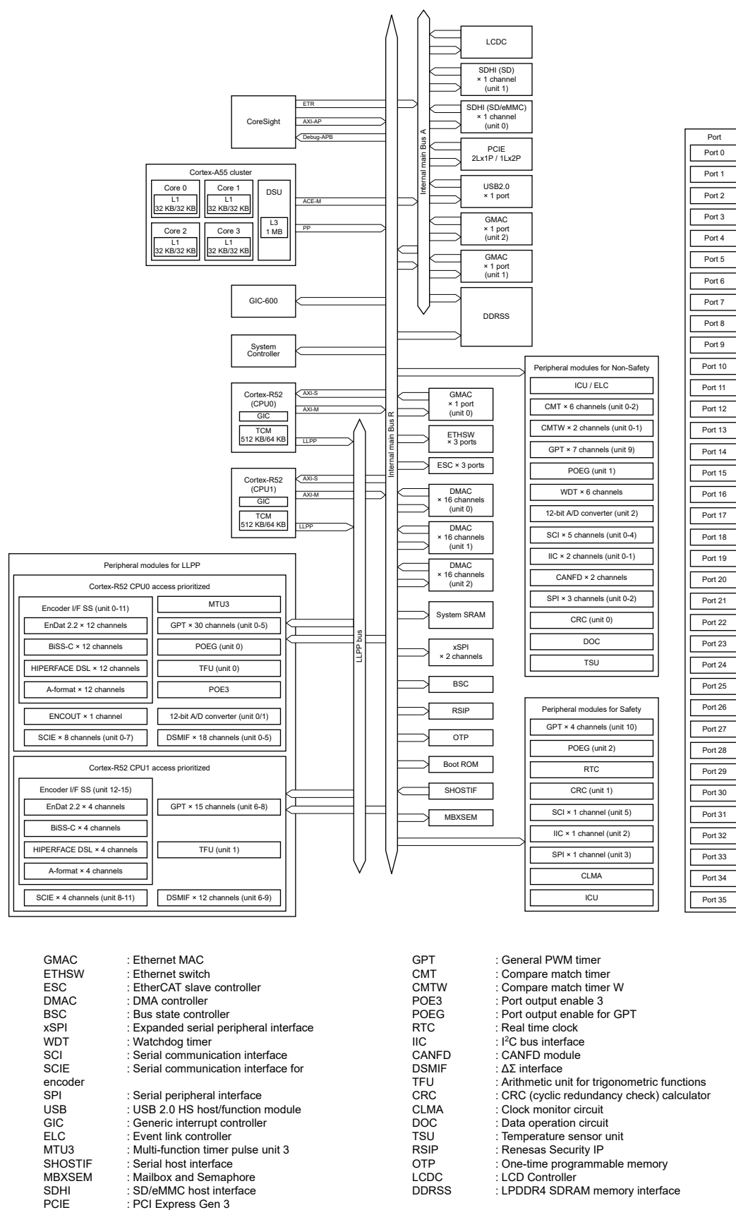
Figure 1.1 Block diagram
