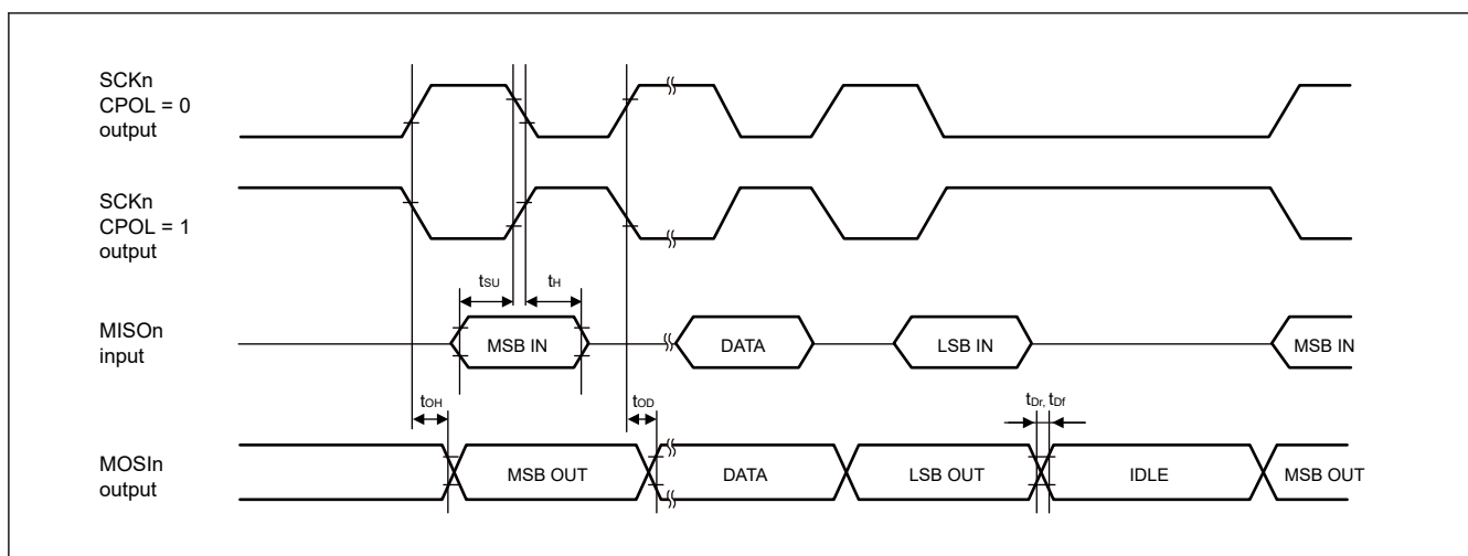
Figure 2.43 SCI simple SPI mode timing for master when CPHA = 1
