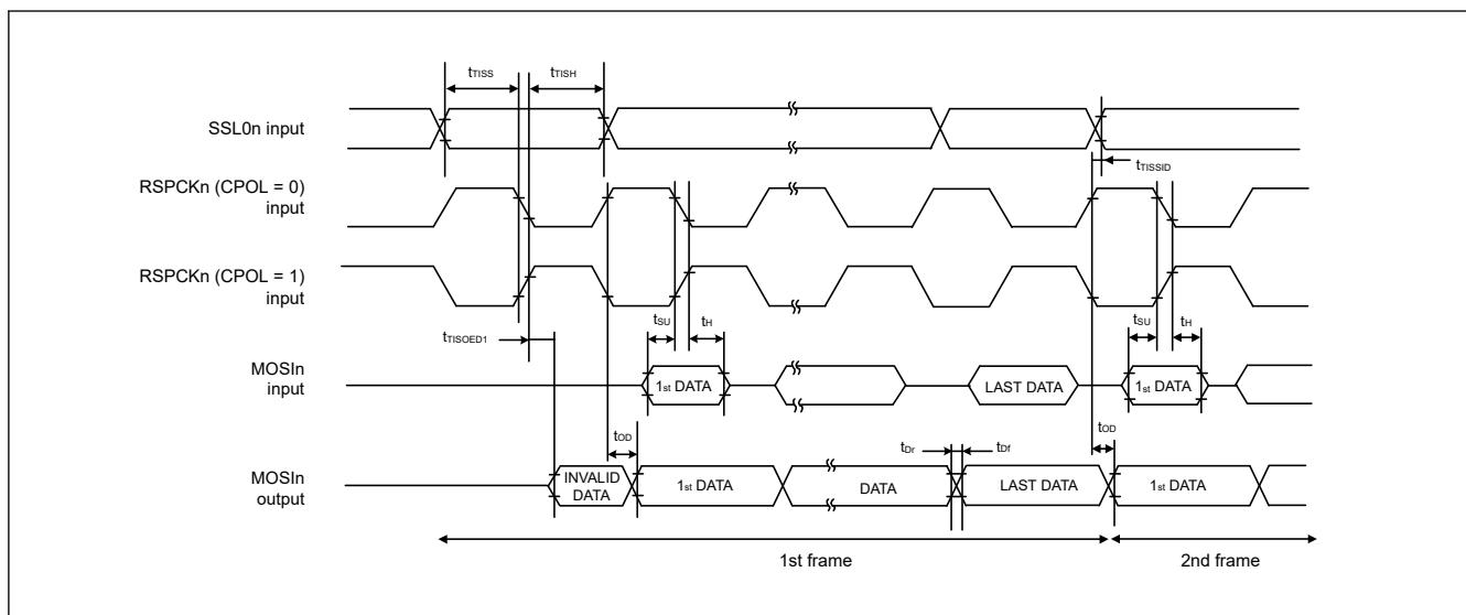
Figure 2.55 SPI timing (Slave, TI-SSP, without delay in burst transfer)
