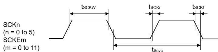
Figure 2.38 SCK clock input/output timing
