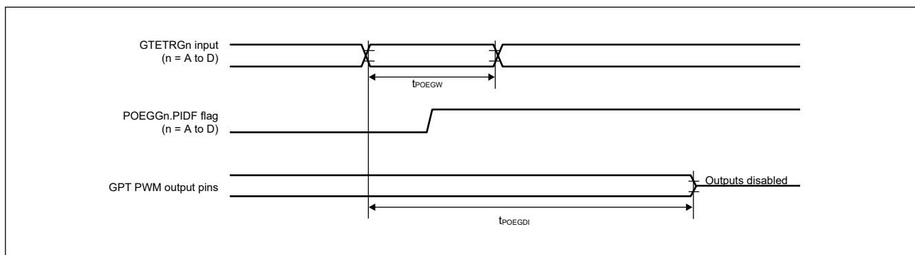
Figure 2.33 Output disable time for POEG via detection flag in response to the input level detection of the GTETR Gn pin
