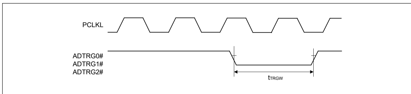
Figure 2.37 A/D converter trigger input timing (ADTRG0#, ADTRG1#, ADTRG2#)
