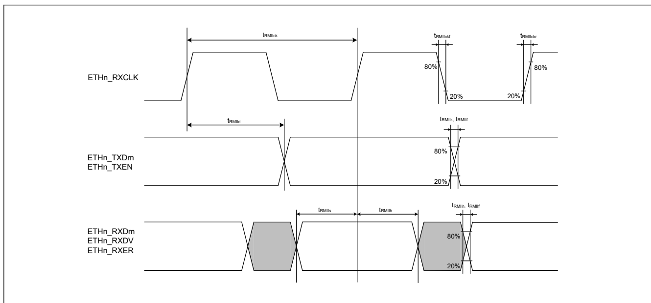
Figure 2.65 RMII transmission and reception timing (n = 0 to 3, m = 0 to 1)
