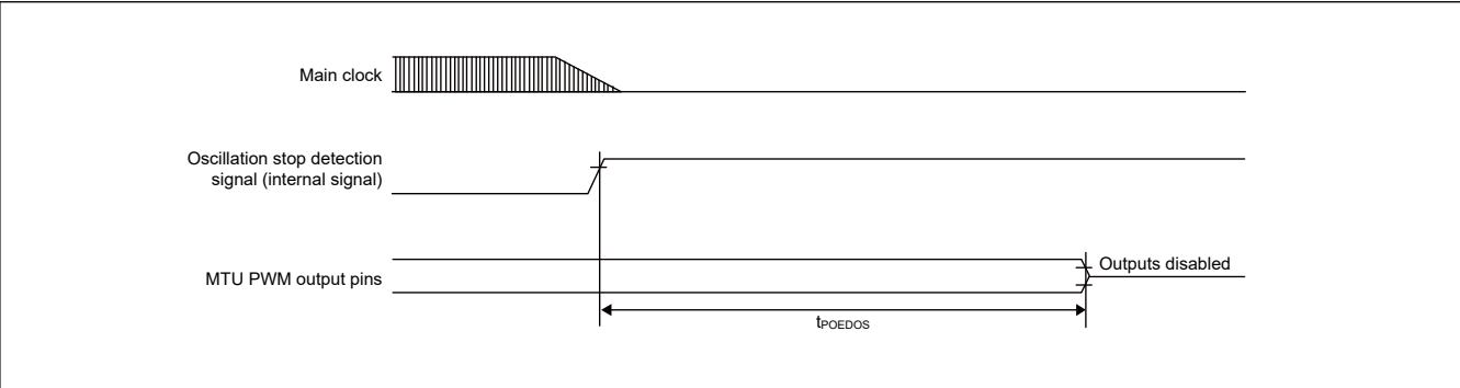
Figure 2.29 Output disable time for POE in response to the oscillation stop detection
