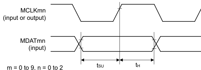
Figure 2.62 Reception timing (MCLKn rising synchronous)
