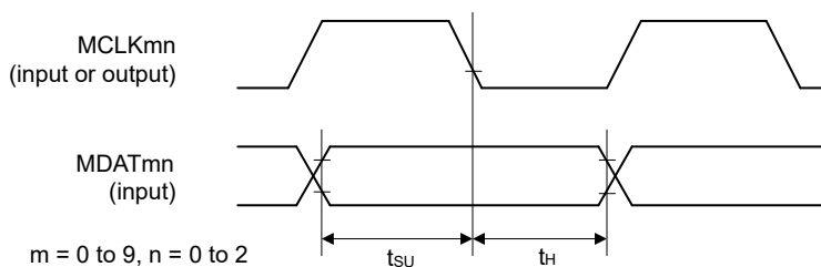
Figure 2.63 Reception timing (MCLKn falling synchronous)
