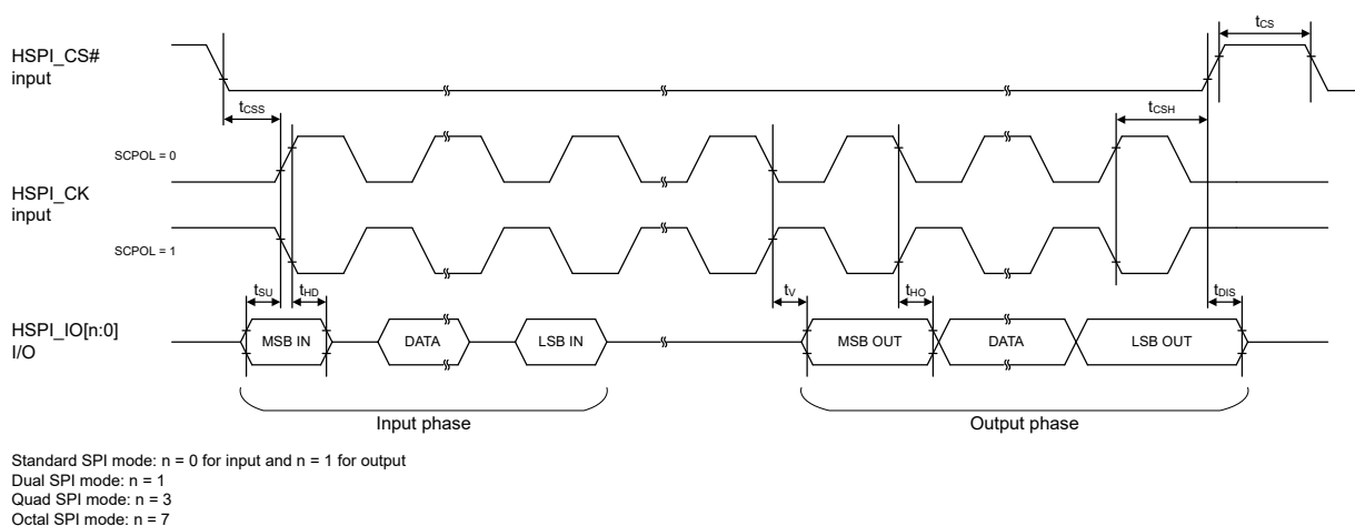
Figure 2.69 SHOSTIF timing (SCPH = 0)
