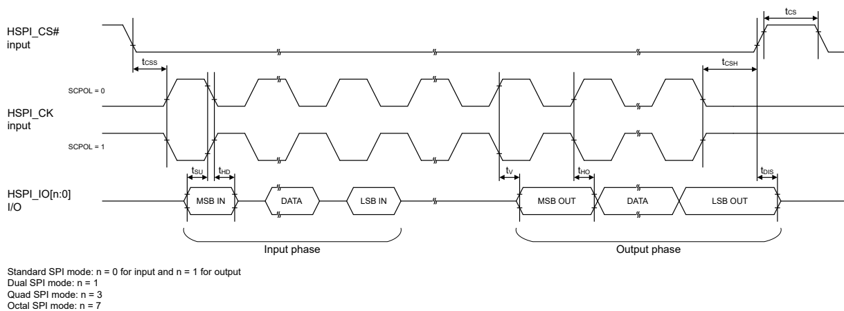
Figure 2.70 SHOSTIF timing (SCPH = 1)
