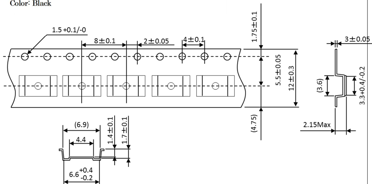
Figure 15: Taping Drawing
