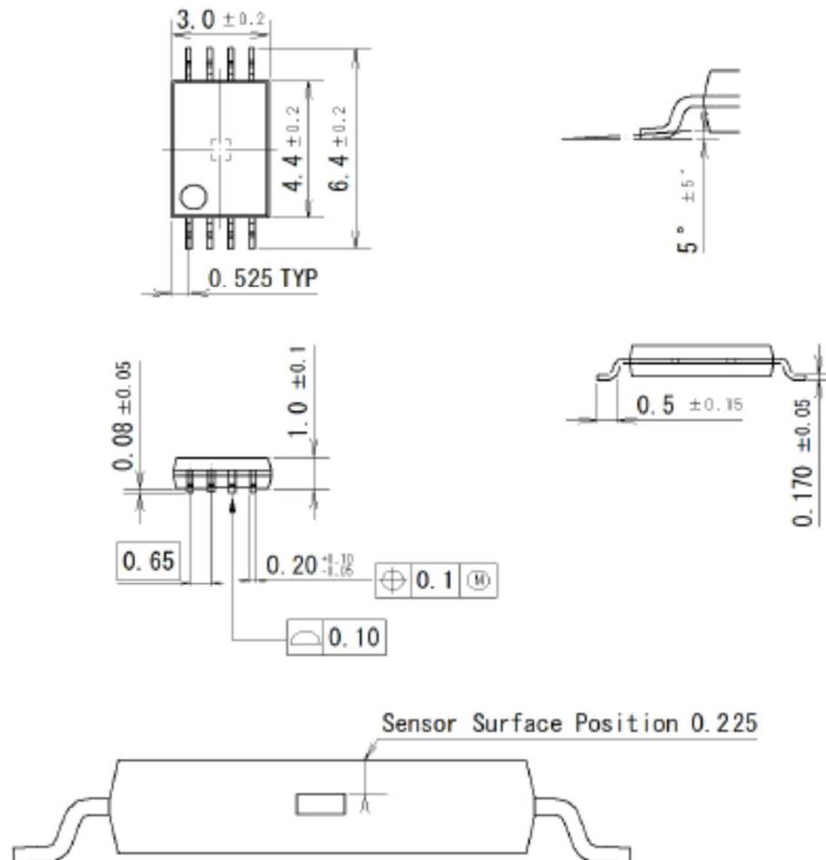
Figure 8: Package drawing
