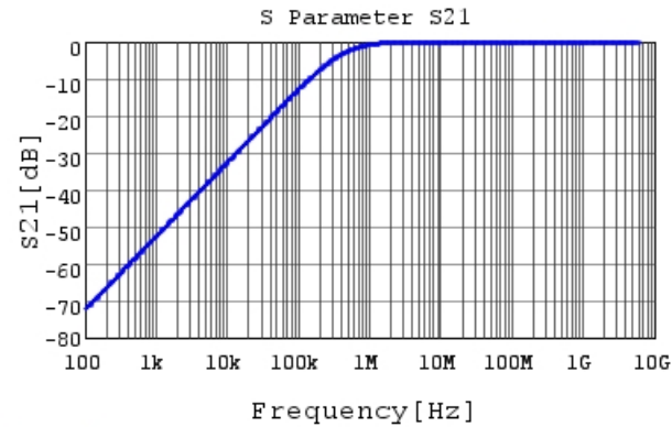
GRM155R71H392KA01 S21 DC0V, 25degC
