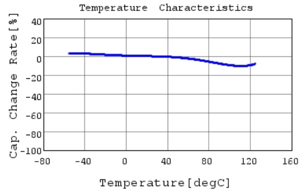
GRM155R71H392KA01 C-Temp. capchange, DC0.0V,
