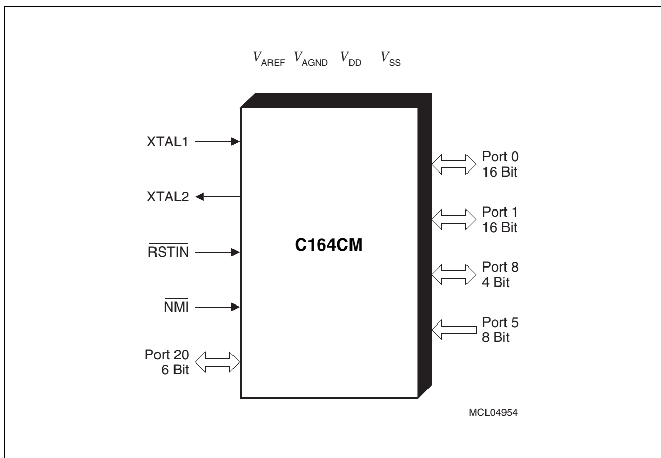
Figure 1 Logic Symbol
