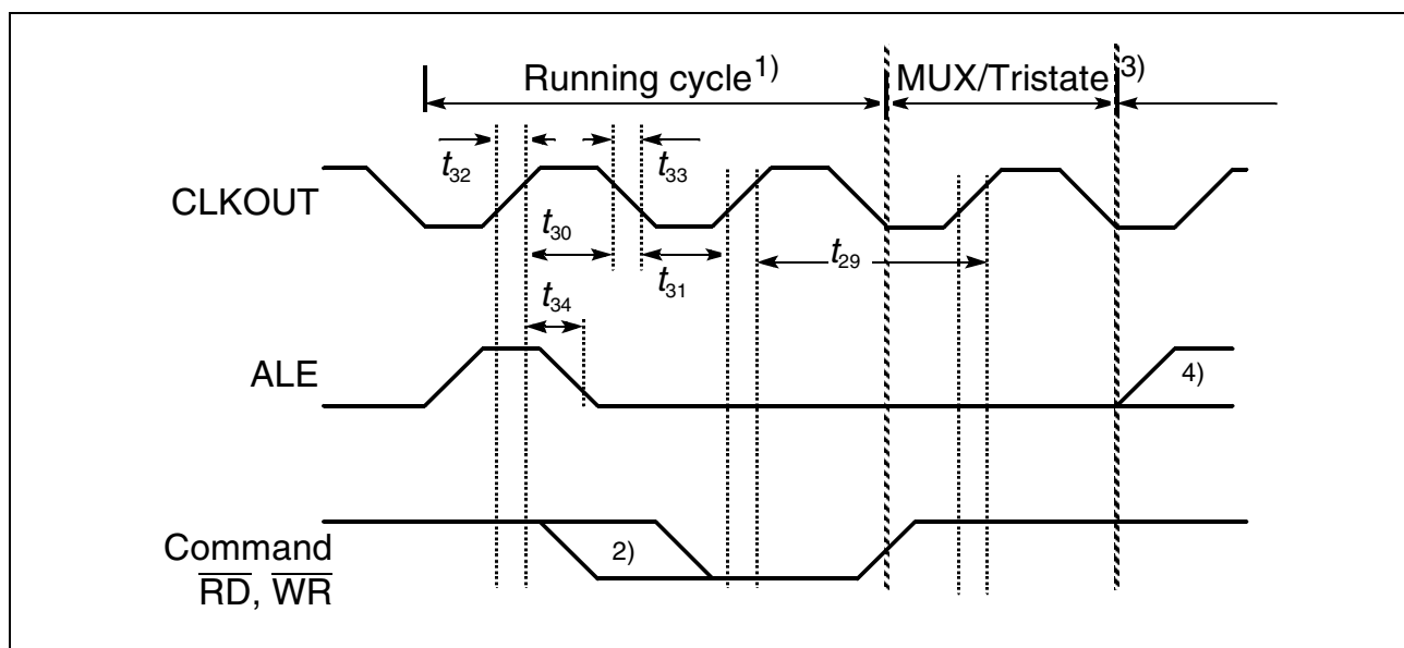
Figure 20 CLKOUT Timing
