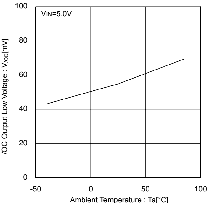
Figure 17. /OC Output Low Voltage vs Ambient Temperature
