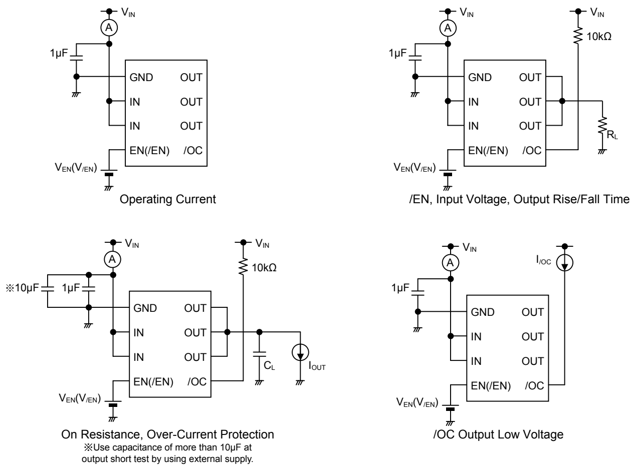
Figure 4. Measurement Circuit
