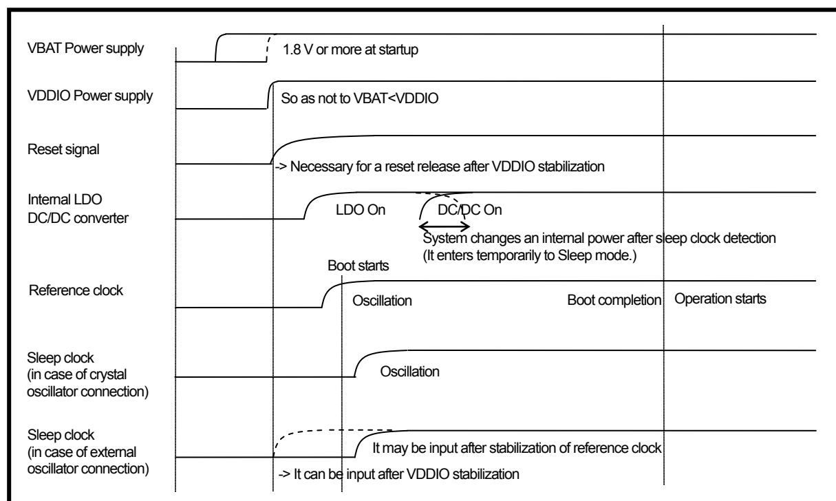
Figure 4-2 Power-on reset release sequence
