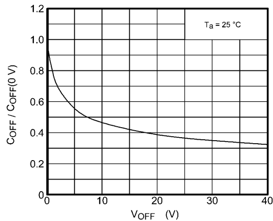
Fig. 12.11 C_{OFF}/C_{OFF}(0\text{ V}) - V_{OFF}
