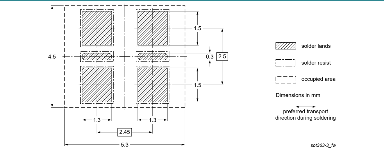
Fig. 14. Wave soldering footprint for TSSOP6 (SOT363-3)
