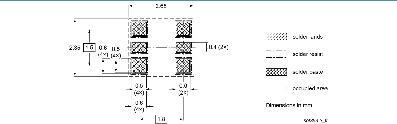
Fig. 13. Reflow soldering footprint for TSSOP6 (SOT363-3)
