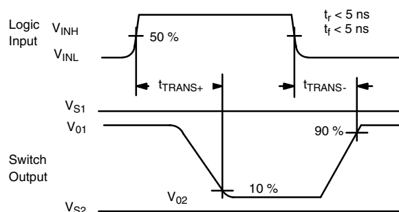
Figure 4. Transition Time
