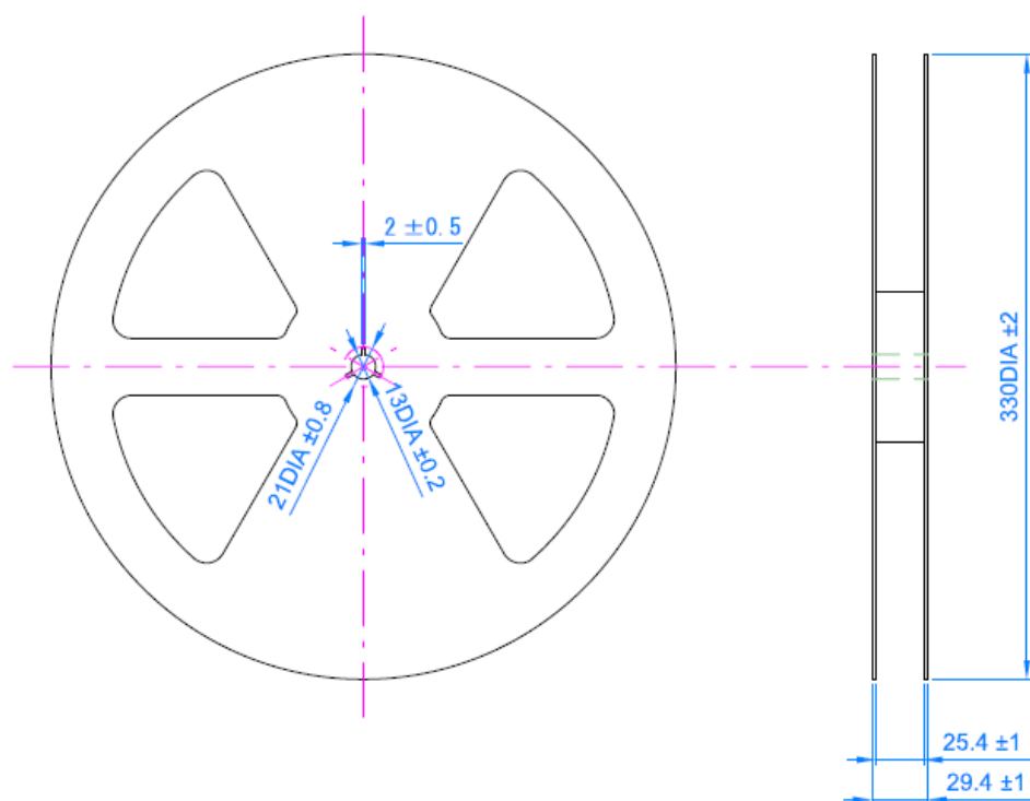
Figure 7-6 Reel dimensions
