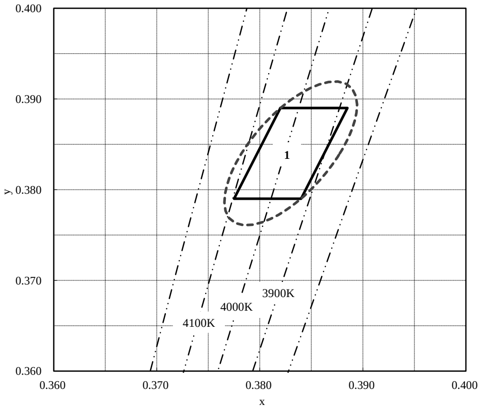
Chromaticity Diagram
