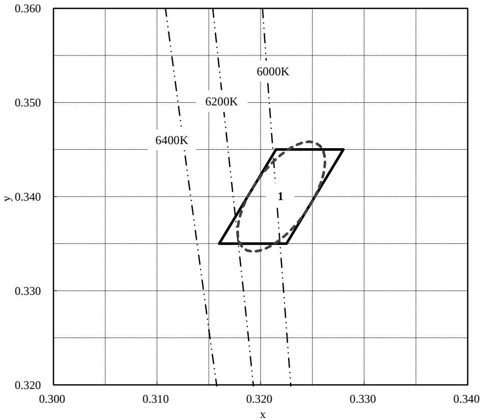
Chromaticity Diagram
