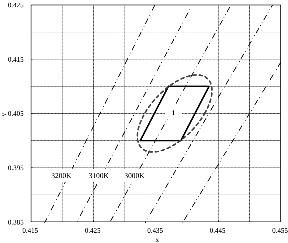
Chromaticity Diagram
