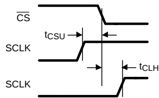
Figure 5. SCLK and \overline{\text{CS}} Timing Parameters
