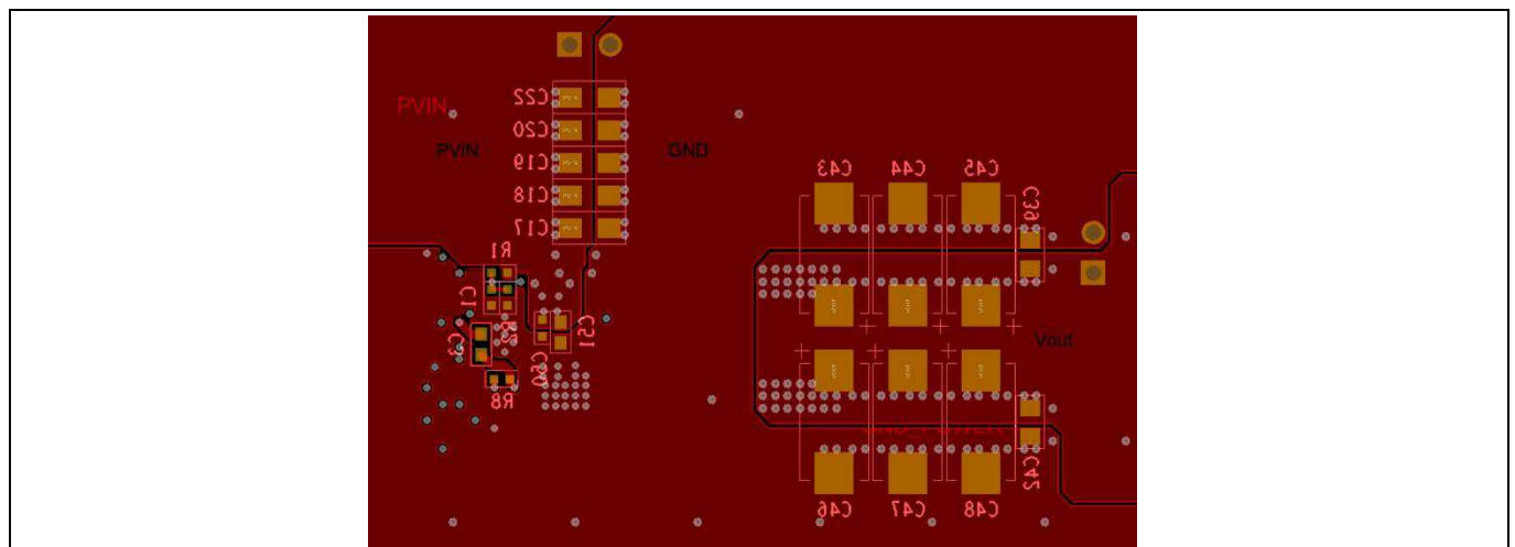
Figure 25 Bottom Layer
