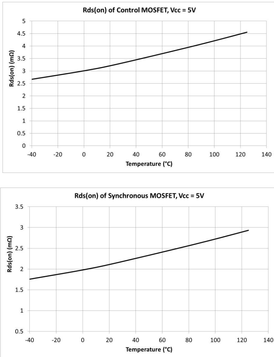
Figure 5 R_{DS(on)} of MOSFETs over Junction Temperature
