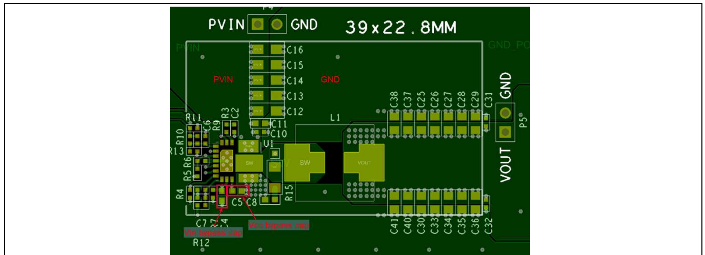
Figure 24 Top Layer
