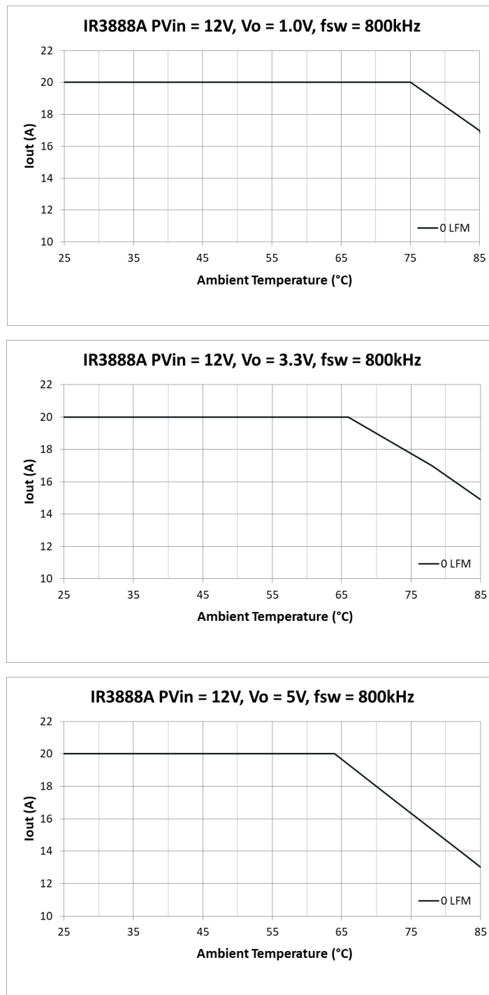
Figure 4 Thermal de-rating curves, P_{Vin} = 12V , V_{out} = 1.0V/3.3V/5V , f_{sw} = 800kHz , V_{CC} = \text{Internal LDO}
