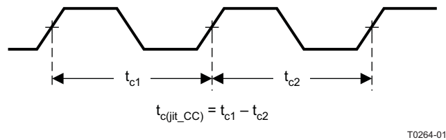
Figure 8. Cycle-to-Cycle Jitter
