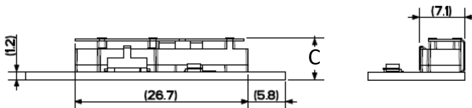
Side View
