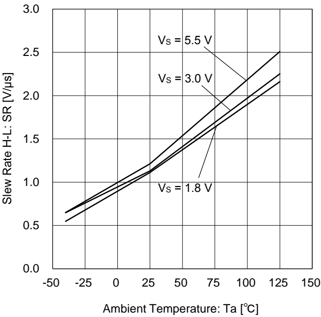
Figure 22. Slew Rate (H to L) vs Ambient Temperature
