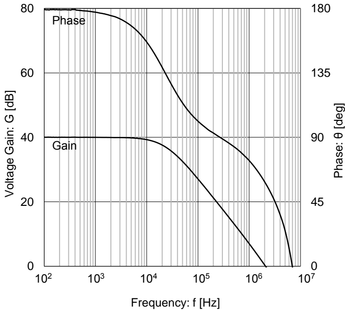
Figure 23. Voltage Gain/Phase vs Frequency (V S = 3.0 V)
