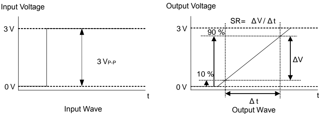
Figure 26. Slew Rate
