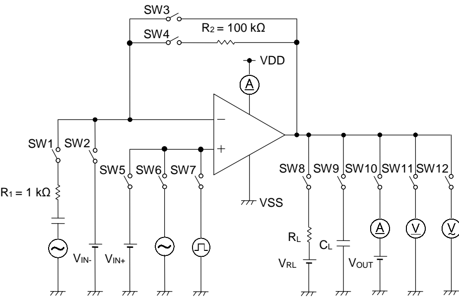
Figure 25. Test Circuit 2
